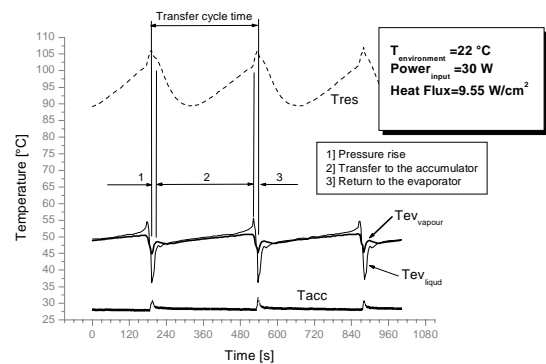
Figure 16 – Temperature diagram for B-device, heat transport regime at 30 W as heat power rate.
