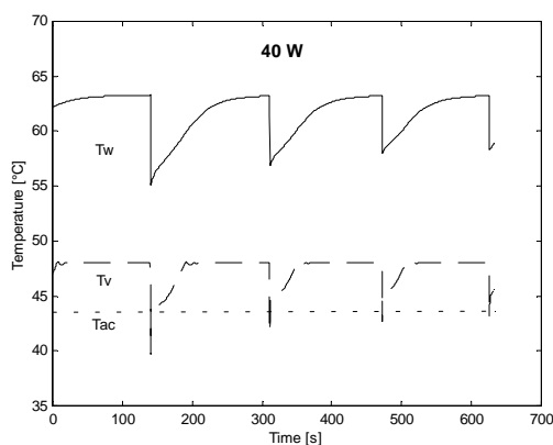
Figure 3 – Temperature diagram for A-device.
