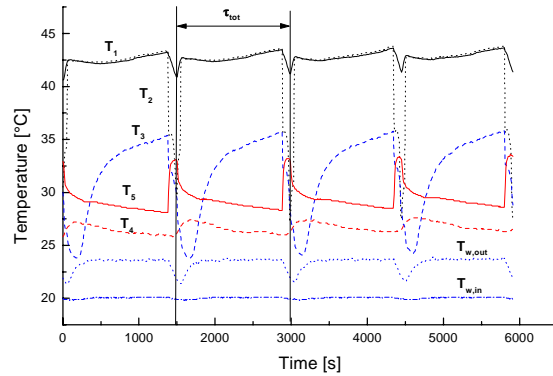
Figure 2 - Temperatures for 4 heat transport cycles in a PTPT.
