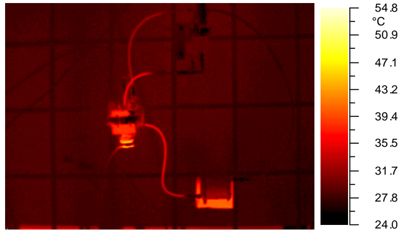
Figure 11 – Infrared thermographic photo of the apparatus during its functioning
