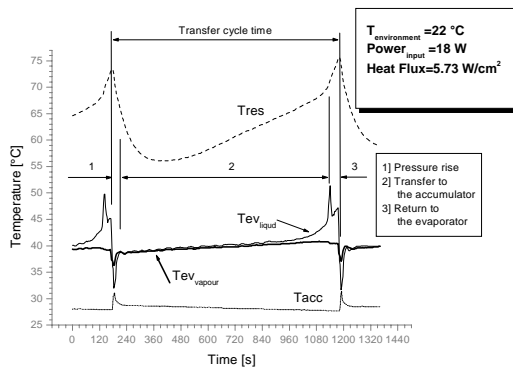
Figure 15 – Temperature diagram for B-device, heat transport regime at 18 W as heat power rate.
