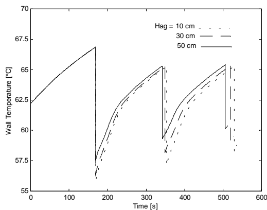
Figure 7 – Influence of the heat flux on the wall evaporator temperatures for A-device.
