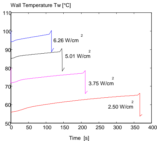
Figure 5 – Influence of the heat flux on the wall evaporator wall temperatures for A-device.
