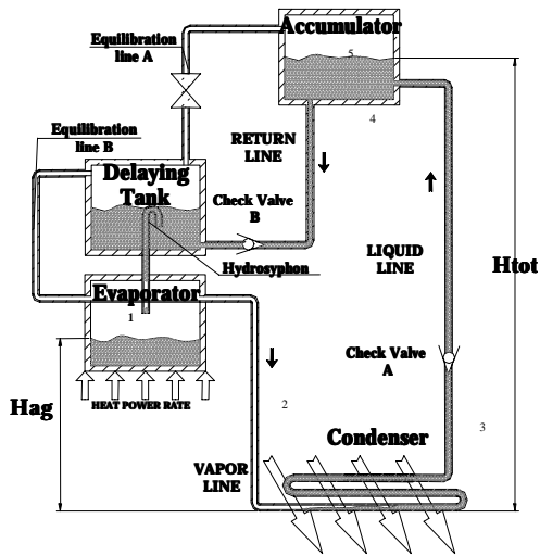
Figure 1 – Functioning scheme of a PTPT.
