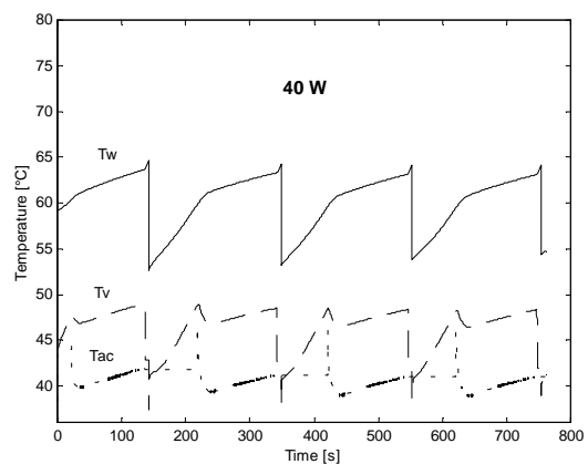
Figure 4 - Temperature diagram for B-device.
