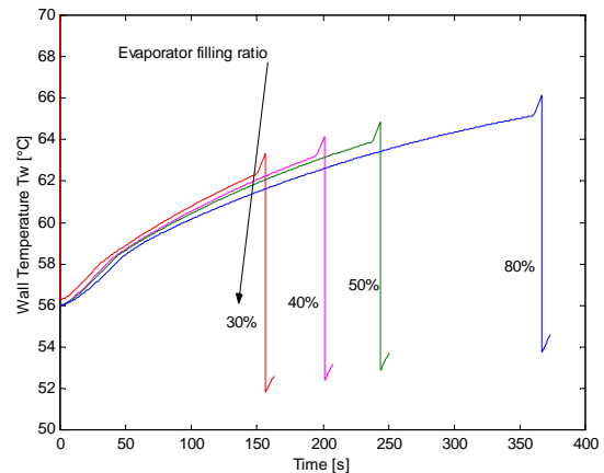
Figure 6 - Influence of the liquid filling ratio on the wall evaporator wall temperatures for A-device..
