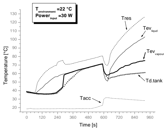
Figure 13 – Experimental start up for A-device
