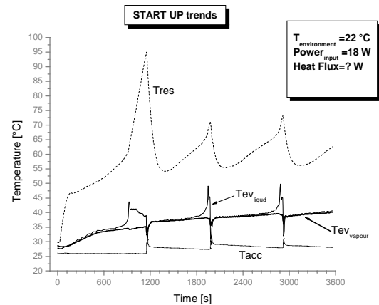
Figure 15 – Temperature diagram for B-device, start up, 18 W as heat power rate.
