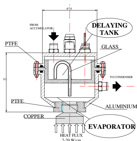
Figure 8 – Evaporator and delaying test.
